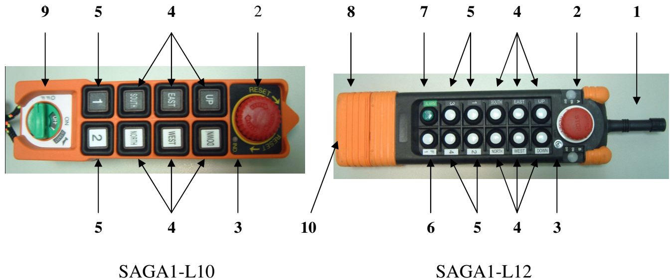
Figure 4-1 Transmitter Configuration
